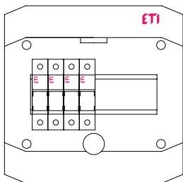
Panel type ECH-8 Fuse disconnecter type: VLC 10
