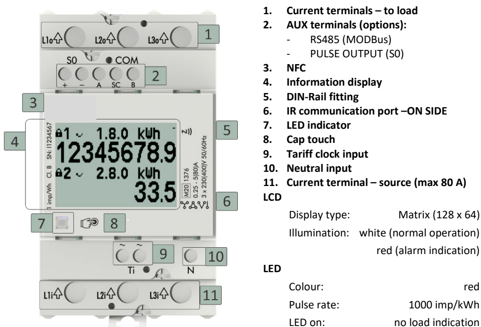
Figure 1: Appearance of three-phase electric energy meter 3MEM80
